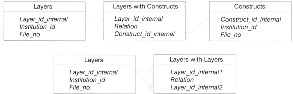
Figure 2. Implementation of many-to-many relationships using link tables. The upper part shows linking between entities, and the lower part linking within entities.
